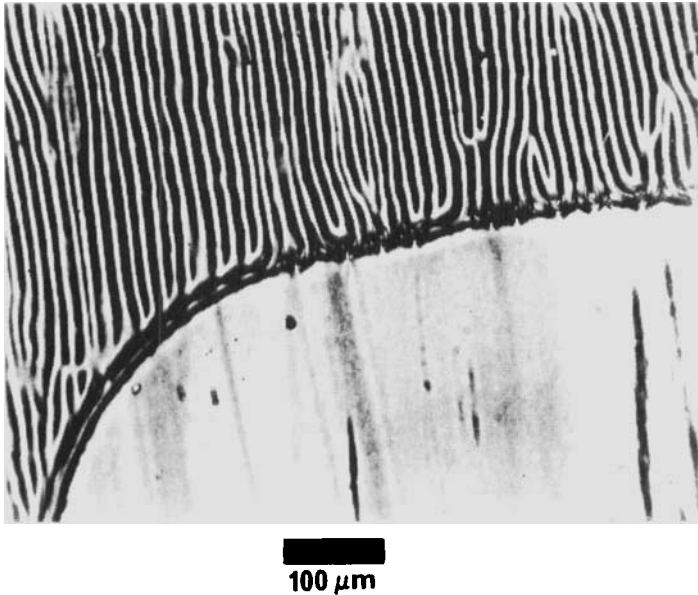
FIGURE 6 Behavior of domains near an edge.
