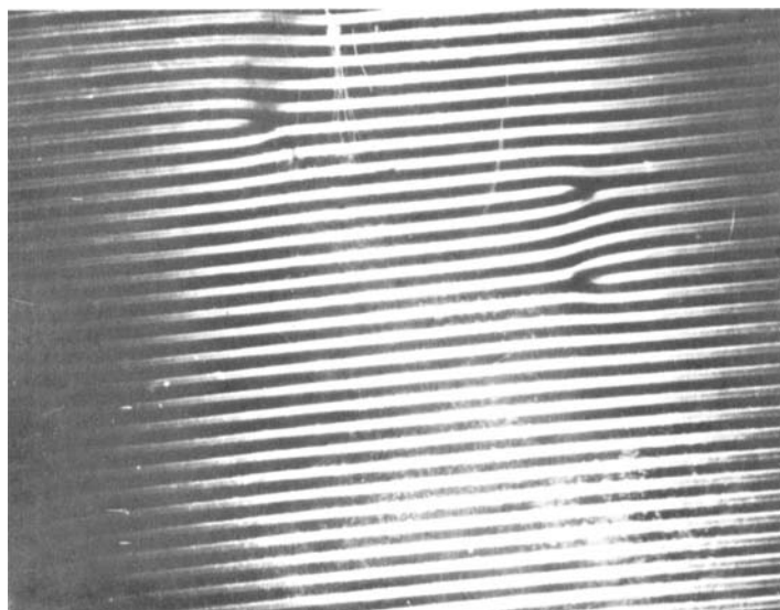
FIGURE 4 The phase grating structure of the VGM device at a fixed voltage viewed through a phase contrast microscope.
