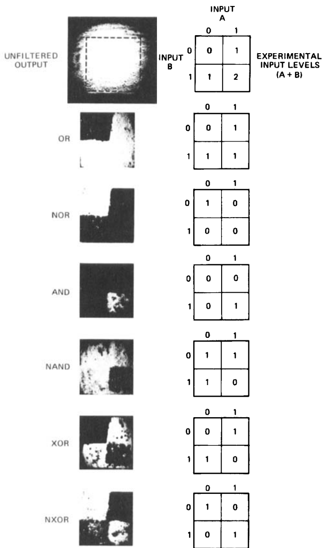
FIGURE 11 VGM logic results. The right-hand column indicates ideal output levels for an image consisting of four quadrants corresponding to truth table values. The left-hand column shows the corresponding experimental results. The first row shows the input for all experiments which consisted of a superposition of two binary images. Succeeding rows show results for the logic operations OR, NOR, AND, NAND, XOR, and NXOR, respectively.
