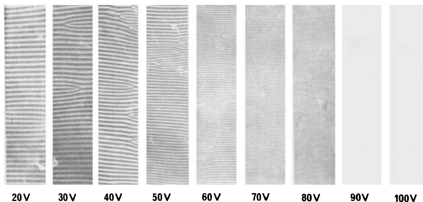
FIGURE 1 VGM viewed through polarizing microscope.
