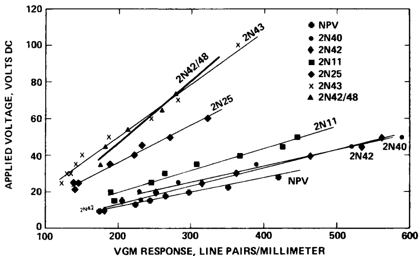
FIGURE 3 VGM voltage dependence for various liquid crystals.
